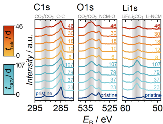
Figure 4. XPS detail spectra for a) C 1s, b) O 1s, and c) Li 1s. Spectra collected from the pristine cathode (bottom, dark blue), cathodes stored at OCV for up to t_{\text{OCV}} = 107 d (turquoise), and those held at U_{\text{hold}} for up to t_{\text{hold}} = 46 d (yellow to red) are displayed. The numbers next to each curve indicate the exact t_{\text{OCV}} or t_{\text{hold}} for the respective cathodes.
