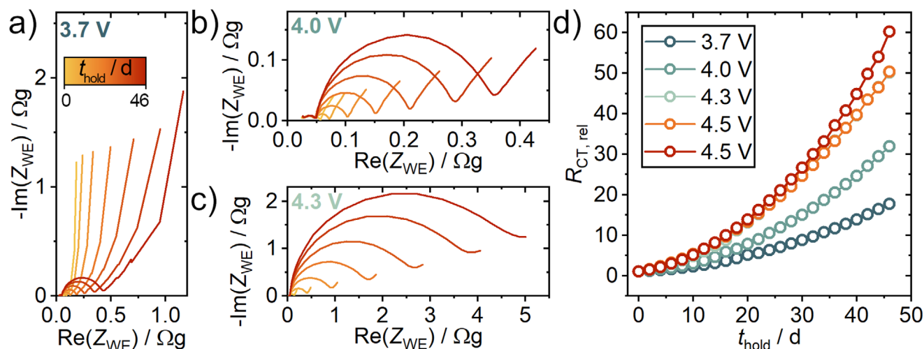
Figure 2. a) EIS data of the cathode impedance ( Z_{\text{WE}} ) at 3.7 V from 1 MHz to 100 \mu\text{Hz} , b) at 4.0 V and c) at 4.3 V from 1 MHz to 100 mHz. The real and imaginary parts of Z_{\text{WE}} are given in \Omega g_{\text{CAM}} , as they are scaled with the mass of active material ( m_{\text{CAM}} ) in the cathode. d) Relative increase of R_{\text{CT}} ( R_{\text{CT,rel}} ) determined by EIS measured at different potentials after holding steps. The orange curve is after 4 h at U_{\text{hold}} , the red one after 48 h. R_{\text{CT,rel}} is calculated from the first recorded R_{\text{CT}} value and R_{\text{CT}} after t_{\text{hold}} via R_{\text{CT,rel}}(t_{\text{hold}}) \equiv R_{\text{CT}}(t_{\text{hold}}) / R_{\text{CT}}(t_{\text{hold}} = 0 \text{ d}) . For the absolute R_{\text{CT}} values refer to Figure S4 (Supporting Information).
