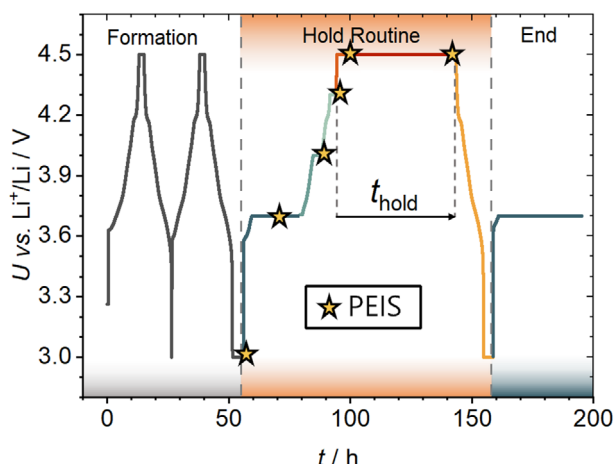
Figure 11. Schematic of the applied electrochemical procedure. All galvanostatic charge steps were performed at 0.1 C, corresponding to 200 mAh g -1 . Left side: Formation from 3.0–4.5 V including a 2 h hold at 4.5 V and a final 4 h hold at 3.0 V. Middle: Hold routine starting with PEIS1 (see text for detailed EIS settings), charge to 3.7 V and hold 2 h, then PEIS2 at 3.7 V, then charge to 4.0 V, hold for 2 h, PEIS (EIS1), charge to 4.3 V, hold for 2 h, PEIS1, charge to 4.5 V, hold for 4 h, PEIS1, hold for further 44 h and PEIS1. Then, discharge to 3 V and hold for 4 h. This routine is repeated. Right: End routine. After completing the desired number of repetitions of the hold routine the cell was charged to 3.7 V, held there for 12 h and then left resting until the cell was disassembled (within 48 h).
